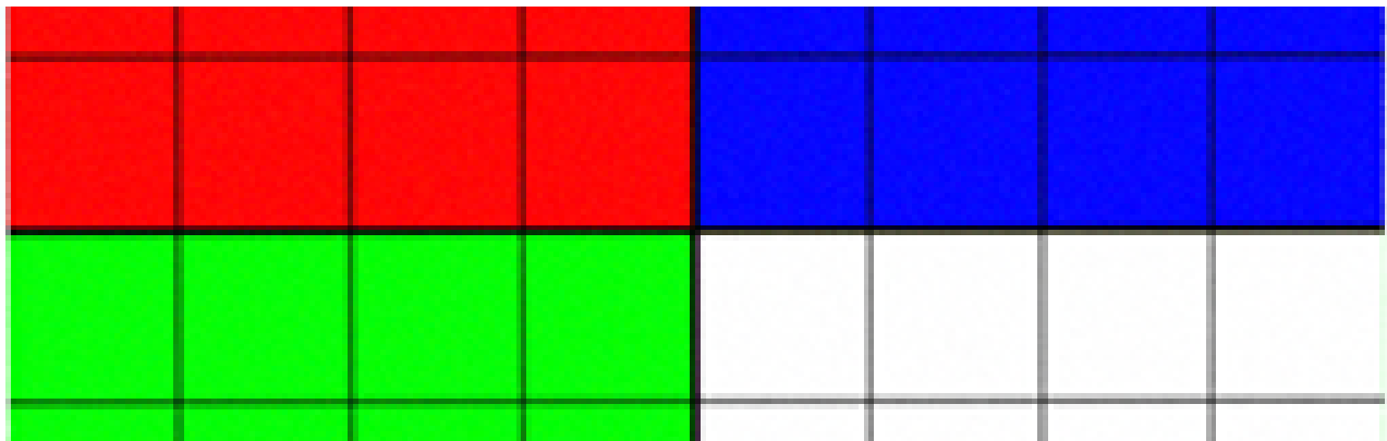
bias = 0
