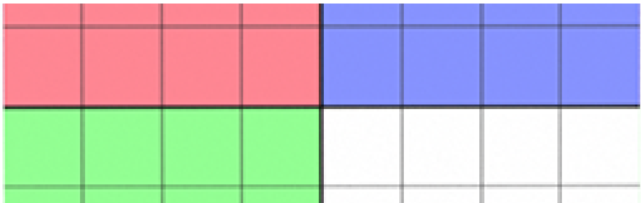
bias = 0.25
